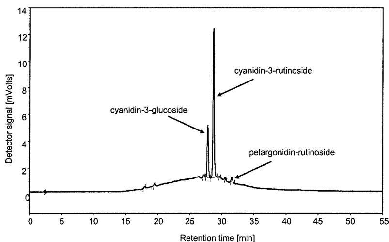
Figure 2. HPLC separation of anthocyanins with açai pulp of 1998 taken as an example. Vis detection at 525 nm.
